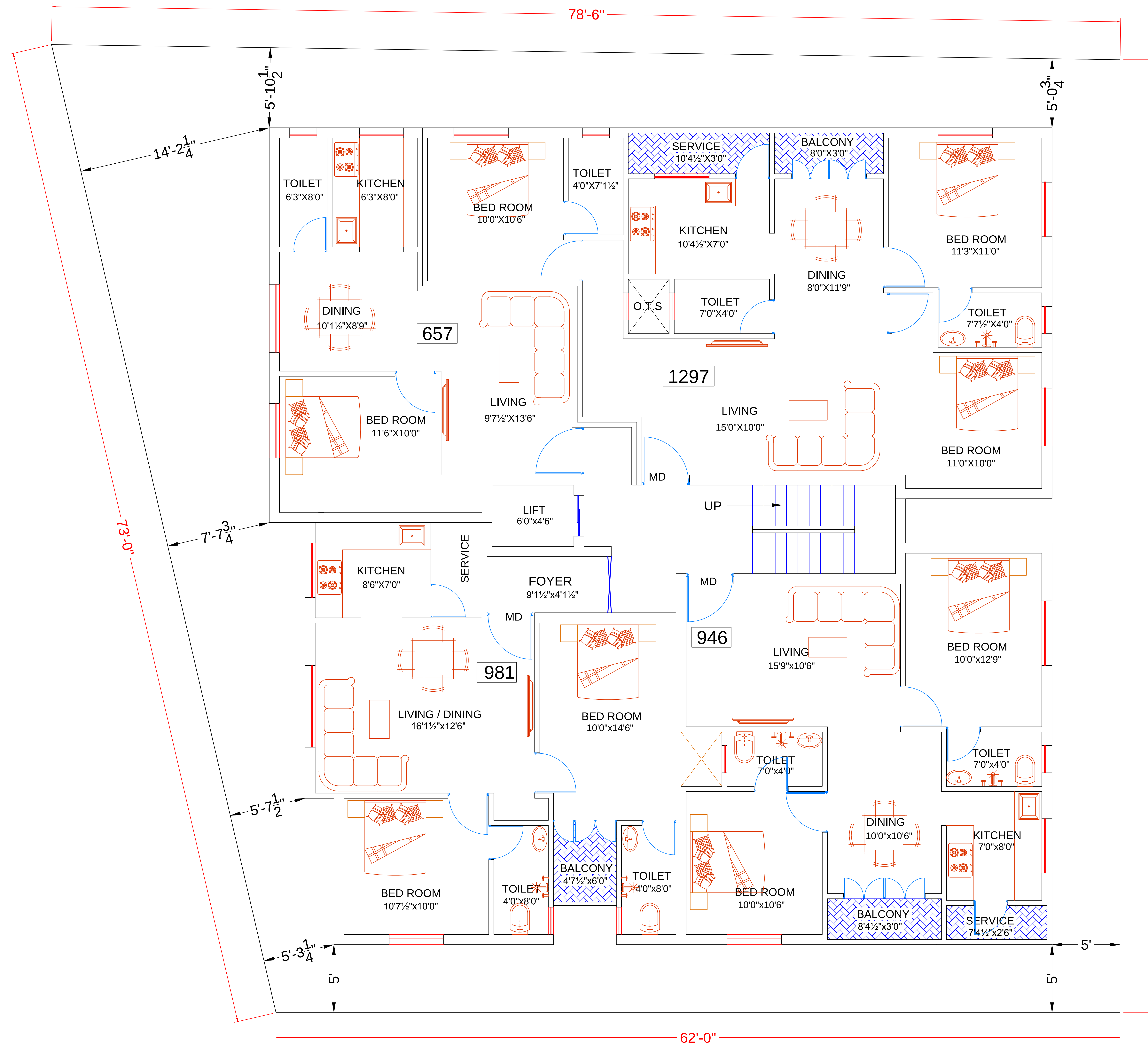
TYPICAL FLOOR PLAN
